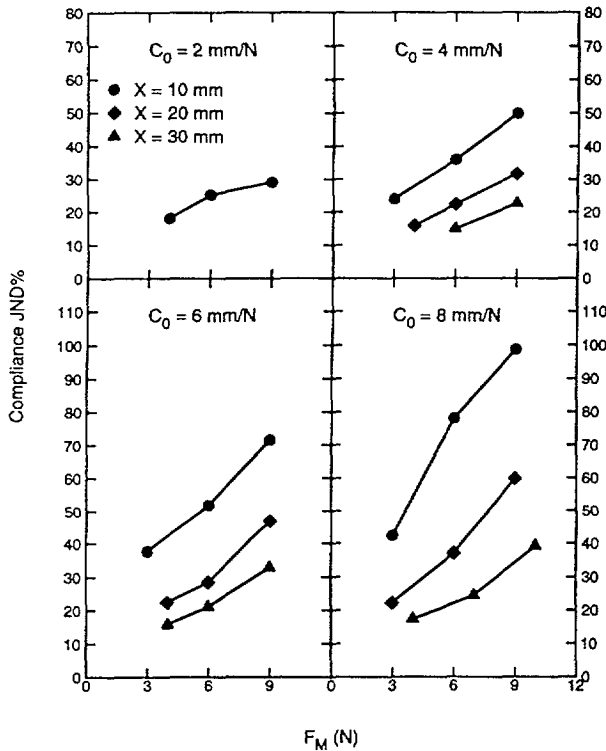
Figure 13. Average compliance JND% results of Experiment 3. The average data from Figure 12 are replotted here to show the effect of displacement X on compliance JND%.
