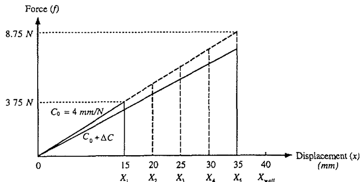
Figure 5. Force-displacement profile for Experiment 2A. Solid lines show two stimuli with C_0 and C_0 + \Delta C that differ in displacement (15 and 35 mm, respectively). Dotted lines show the rest of the 10 possible force-displacement profiles associated with C_0 , C_0 + \Delta C , and X_i ( i = 1, 2, \dots, 5 ).
