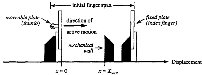
Figure 2. Diagram illustrating the layout of the apparatus.
