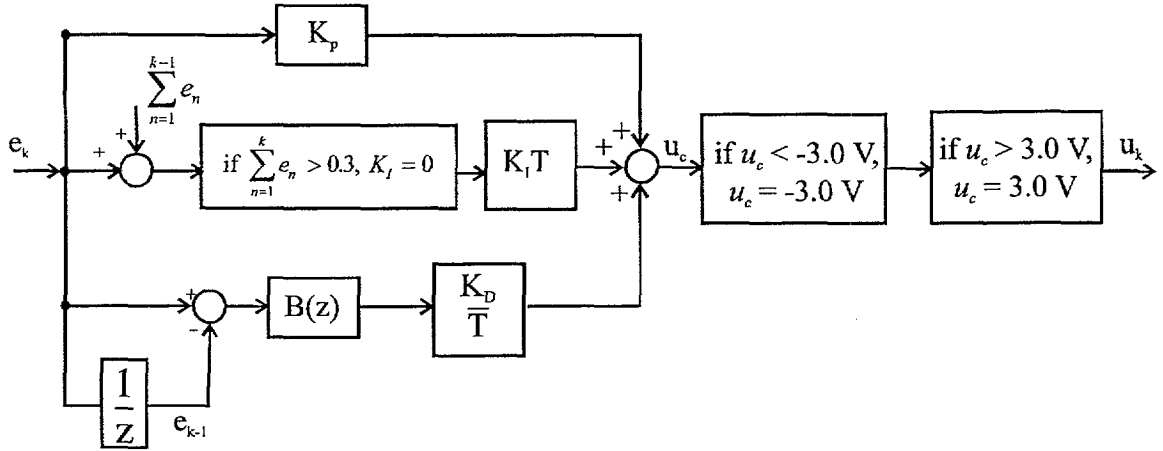
Figure 3.6: Signal Flow Diagram of the Controller
