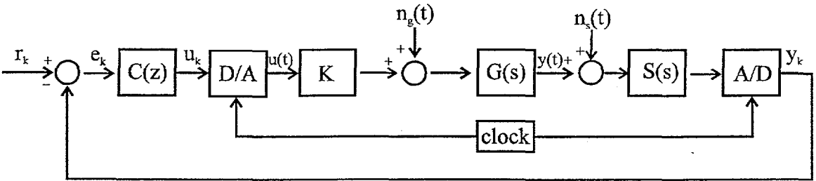
Figure 3.5: Signal Flow Diagram Representing Position Control
